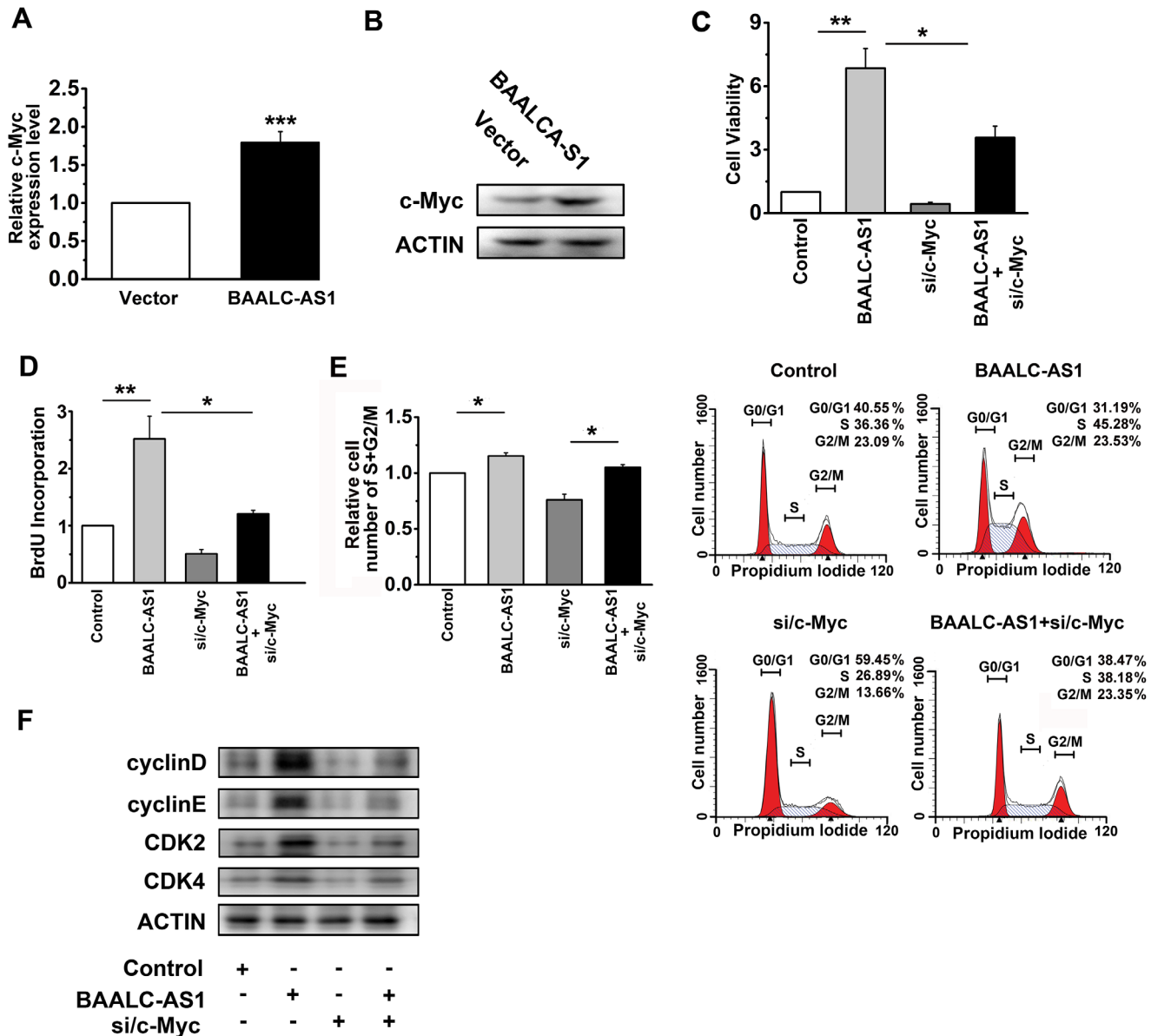
FIGURE 7 BAALC-AS1 promotes cell proliferation by up-regulating c-Myc. A , Expression of c-Myc quantified by RT-qPCR after BAALC-AS1 overexpression in KYSE-450 cells. B , Western blotting analyses of the protein expression levels of c-Myc after BAALC-AS1 overexpression in KYSE-450 cells. C , MTS assay was used to determine the viability of KYSE-450 cells transfected with BAALC-AS1 overexpression plasmids and c-Myc siRNAs. D , BrdU incorporation showed the synthesis of DNA in KYSE-450 cells transfected with BAALC-AS1 overexpression plasmids and c-Myc siRNAs. E , Flow cytometry were performed to determine the percentage of cells in S and G2/M phases in KYSE-450 cells transfected with BAALC-AS1 overexpression plasmids and c-Myc siRNAs. F , Western blotting analyses of the protein expression levels of Cyclin D, Cyclin E, CDK2, and CDK4 in KYSE-450 cells transfected with BAALC-AS1 overexpression plasmids and c-Myc siRNAs. *, P < 0.05 ; **, P < 0.01 ; ***, P < 0.001 . All values are expressed as the mean \pm SEM.
